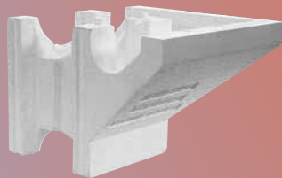
Brick Ledge Corner Block (17" x 17" x 12")
