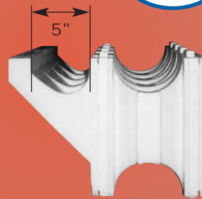
Brick Ledge/Footing Profile
