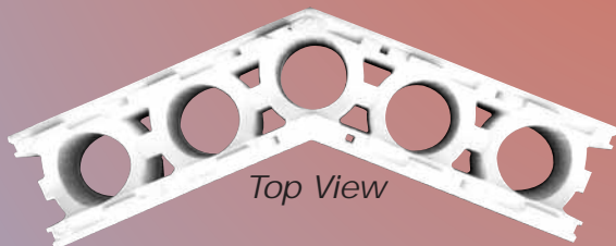
Brick Ledge Corner Block (17" x 17" x 12")
